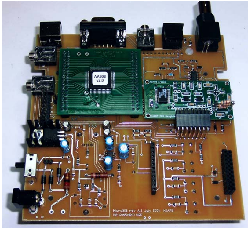
Top/Component Side
