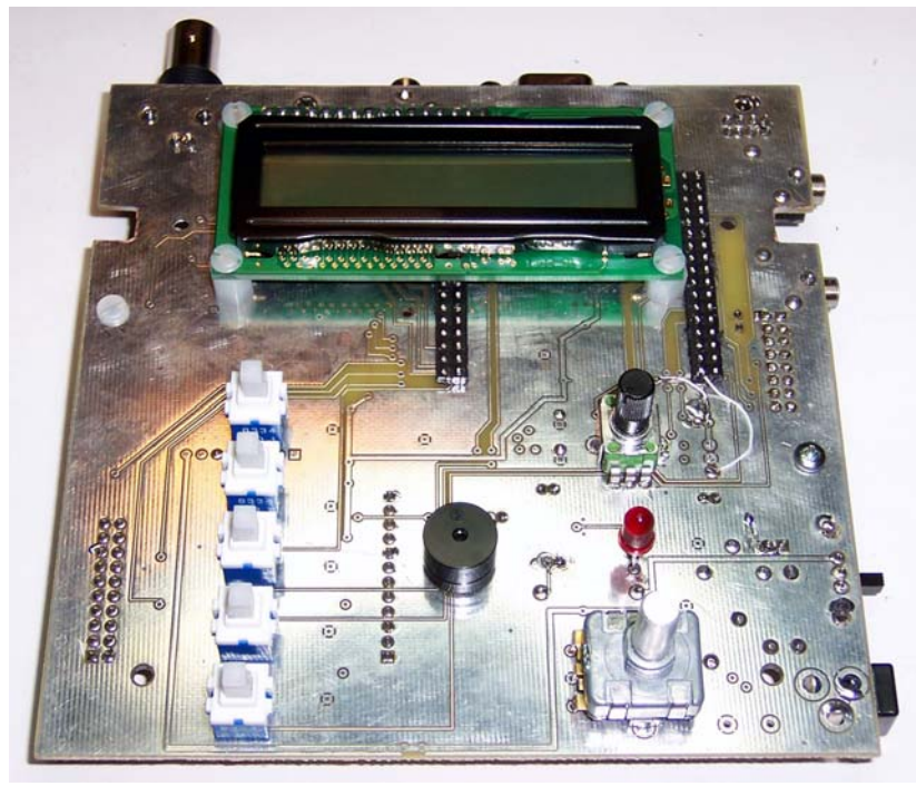
Bottom/Controls Side
